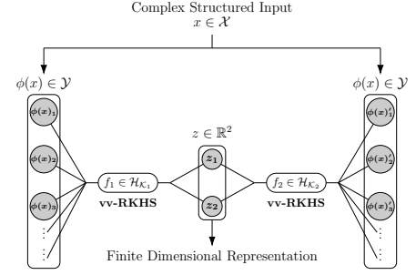
Figure 5. 2-Layer Kernel Autoencoder
