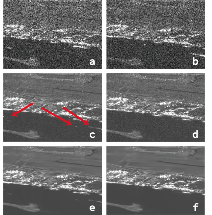
Fig. 4: Geometric vs arithmetic mean: (a) and (b) two images from the time series corresponding to dates t=11 and t=17 , (c) arithmetic mean and (d) debiased geometric mean, (e) denoised arithmetic mean and (f) denoised geometric mean.
