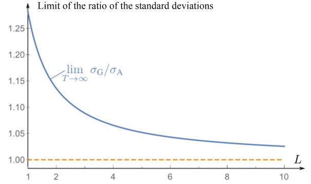
Fig. 1: Ratio \sigma_G/\sigma_A , for large values of T , as a function of the number of looks L .
