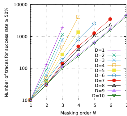
Fig. 4 Number of traces necessary for SR \geq 50\% on n = 8 bits (when \sigma = 1 ), as a function of the masking order N = d + 1 , for several sub-trace dimensionalities D
