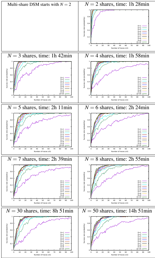
Fig. 10 Attacks on D = 1, \dots, 10 samples for noise \sigma = 1.0 , and various number of shares (for 100 attacks) against (incorrect, see App. A.1) Multi-Share DSM on PRESENT ( n = 4 bit)
