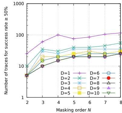
Fig. 6 Number of traces necessary for SR \geq 50\% for incorrect MS-DSM on n = 4 bits (when \sigma = 1 ), as a function of the masking order N = d + 1 , for several sub-trace dimensionalities D
