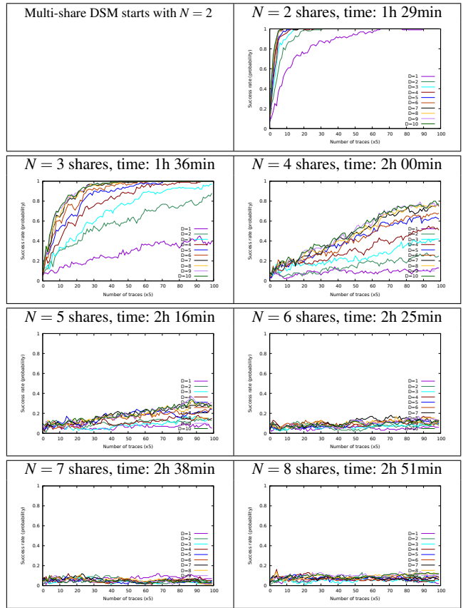
Fig. 11 Attacks on D = 1, \dots, 10 samples for noise \sigma = 1.0 , and various number of shares (for 100 attacks) against (correct, see App. A.2) Multi-shares DSM on PRESENT ( n = 4 bit)
