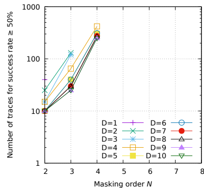
Fig. 7 Number of traces necessary for SR \geq 50\% for correct MS-DSM on n = 4 bits (when \sigma = 1 ), as a function of the masking order N = d + 1 , for several sub-trace dimensionalities D
