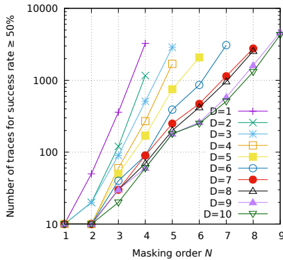
Fig. 5 Number of traces necessary for SR \geq 50\% on n = 4 bits (when \sigma = 1 ), as a function of the masking order N = d + 1 , for several sub-trace dimensionalities D
