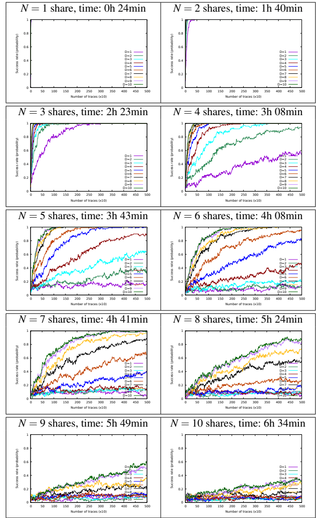
Fig. 9 Attacks on D = 1, \dots, 10 samples on Boolean Masking of PRESENT ( n = 4 bit) for noise \sigma = 1.0 , and various number of shares (for 100 attacks)
