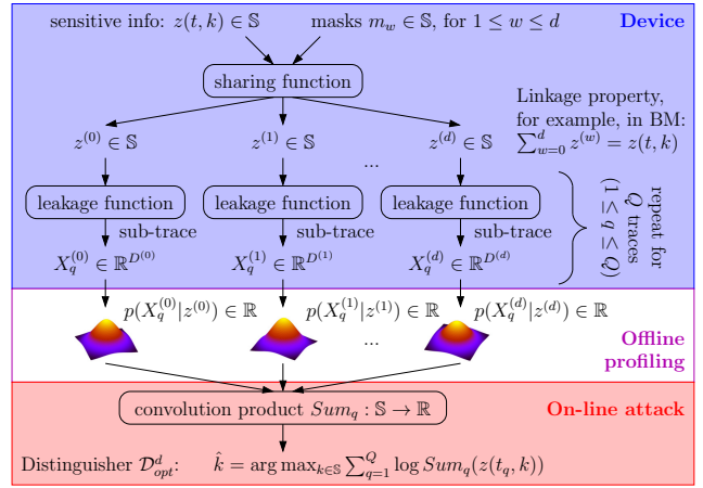
Fig. 1 Synoptic of the multivariate high-order attack, applied on d^{th} -order Boolean Masking (BM)
