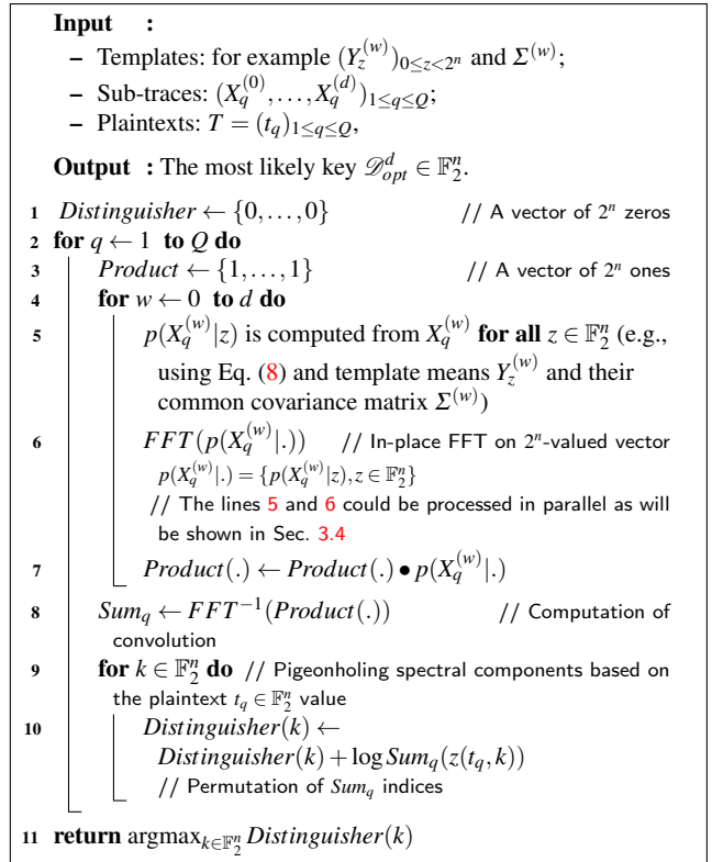
Algorithm 1: H-O Template Attacks with efficient processing.
