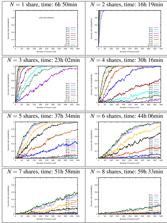
Fig. 8 Attacks on D = 1, \dots, 10 samples on Boolean Masking of AES ( n = 8 bit) for noise \sigma = 1.0 , and various number of shares (for 100 attacks)
