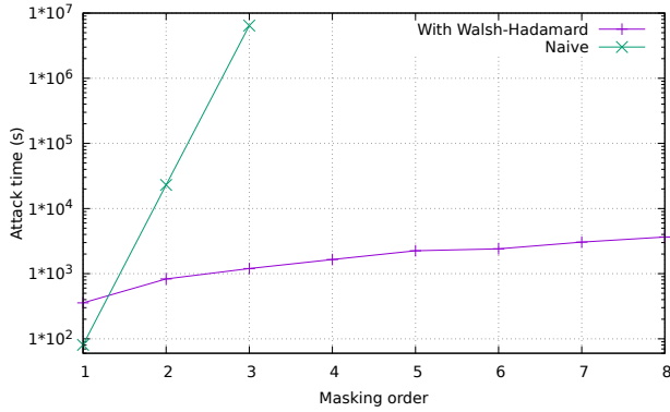
Fig. 2 Single attack time (on 5000 samples), as a function of its order (= number of shares)
