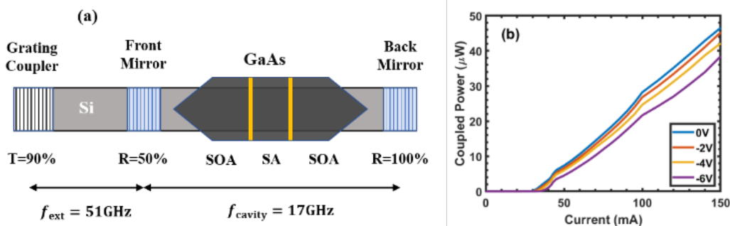
Figure 1: (a) Schematic diagram of the hybrid-silicon QD comb laser. (b) Light-current characteristics of the QD comb laser under different voltages on SA.
