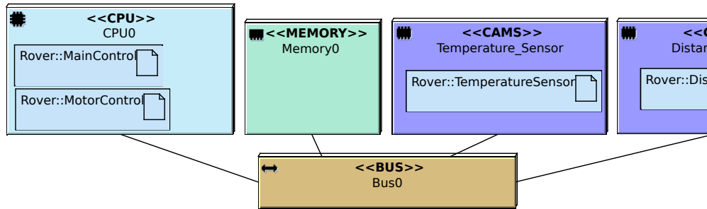
Figure 6. Partitioning level architecture and mapping diagram
