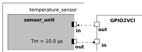
Figure 12. SystemC-AMS representation of the temperature sensor in TTool
