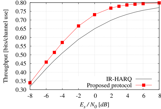
Figure 4: Throughput versus E_s/N_0 (MD, CAC, C = 3 , T = 3 ).
