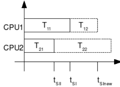
Fig. 4. Scheduling scenario
