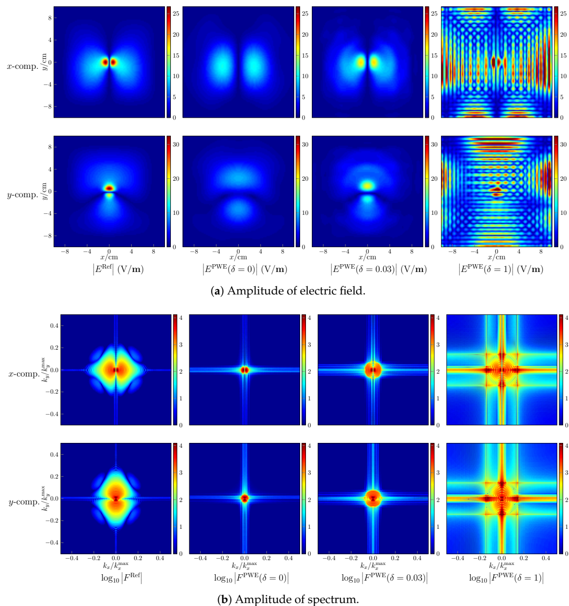
Figure 5. Field reconstruction with respect to the seventh case, |E| denotes the amplitude of electric field, |F| the amplitude of spectrum, and the superscript “PWE”, “Ref” indicate the reconstructed field and the reference field, respectively.
