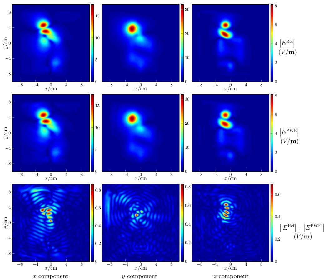
Figure 3. Field reconstruction with respect to the fourth case. E^{\text{PWE}} and E^{\text{Ref}} denote the reconstructed field and the reference field, respectively.
