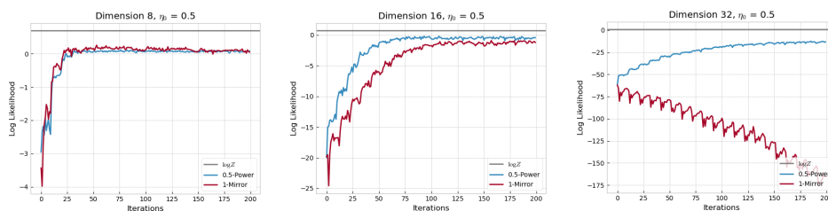
Figure 2: Plotted is the average Log-likelihood for 0.5-Power and 1-Mirror Descent in dimension d = \{8, 16, 32\} computed over 100 replicates with \eta_0 = 0.5 .
