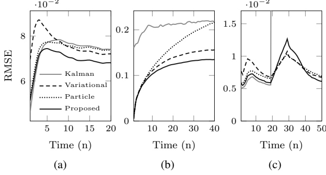
Fig. 2. Linear filtering results given a signal with: (a) Laplace noise, (b) Gaussian outliers, and (c) Gaussian noise of variance 1 for 20 \leq n \leq 30 , and 10^{-4} otherwise.
