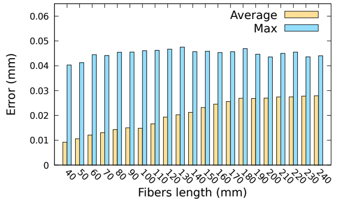
Fig. 8: Error in mm depending on streamlines length for an 8 bits octahedral quantization with \delta = 0.1mm .
