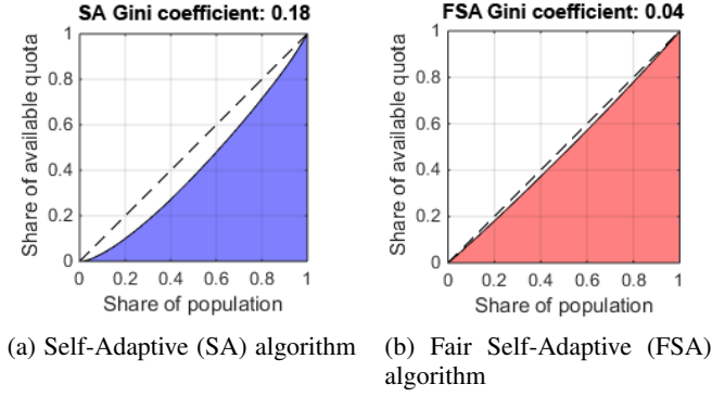
Fig. 9: Lorenz curves and Gini indices analyzing the final distribution of available cellular quota in both algorithms.
