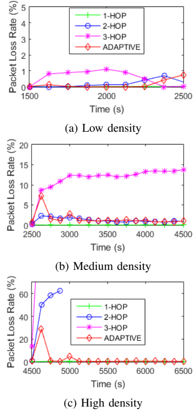
Fig. 5: Packet Loss Rate (PLR) in function of time for the tested scenario. Comparison between 1-, 2- and 3-hop configurations vs. Self-Adaptive algorithm.
