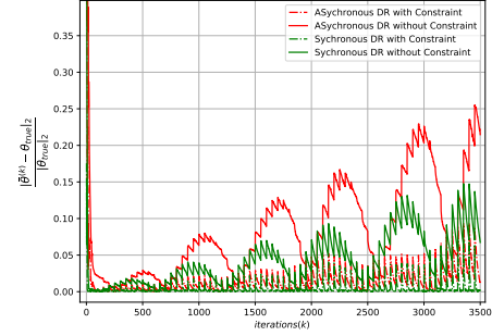
(a) Convergence of solutions against iterations ( k ): \boldsymbol{\theta} represent mean of \boldsymbol{\theta}_v, v = 1, \dots, N , and \boldsymbol{\theta}_{\text{true}} represents true positions of target.
