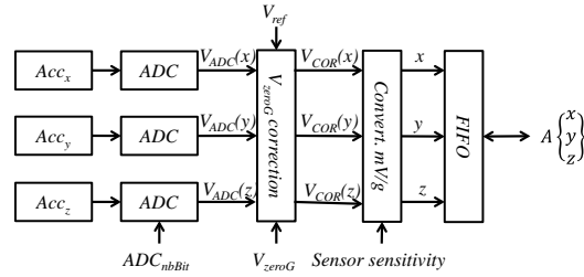
Fig. 8 : Acceleration measuring process
