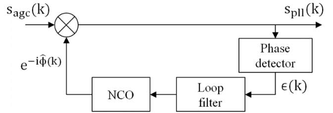
Figure 2. Block diagram of the digital phase-locked loop
