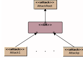
Fig. 3. OR operator
