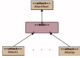
Fig. 2. AND operator
