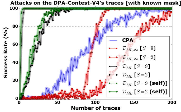
Fig. 7. Comparison of success rate of CPA, \mathcal{D}_{ML,sto} for S \in \{9, 2\} , and \mathcal{D}_{ML} for S \in \{9, 2\} (with two distinct learning methods)
