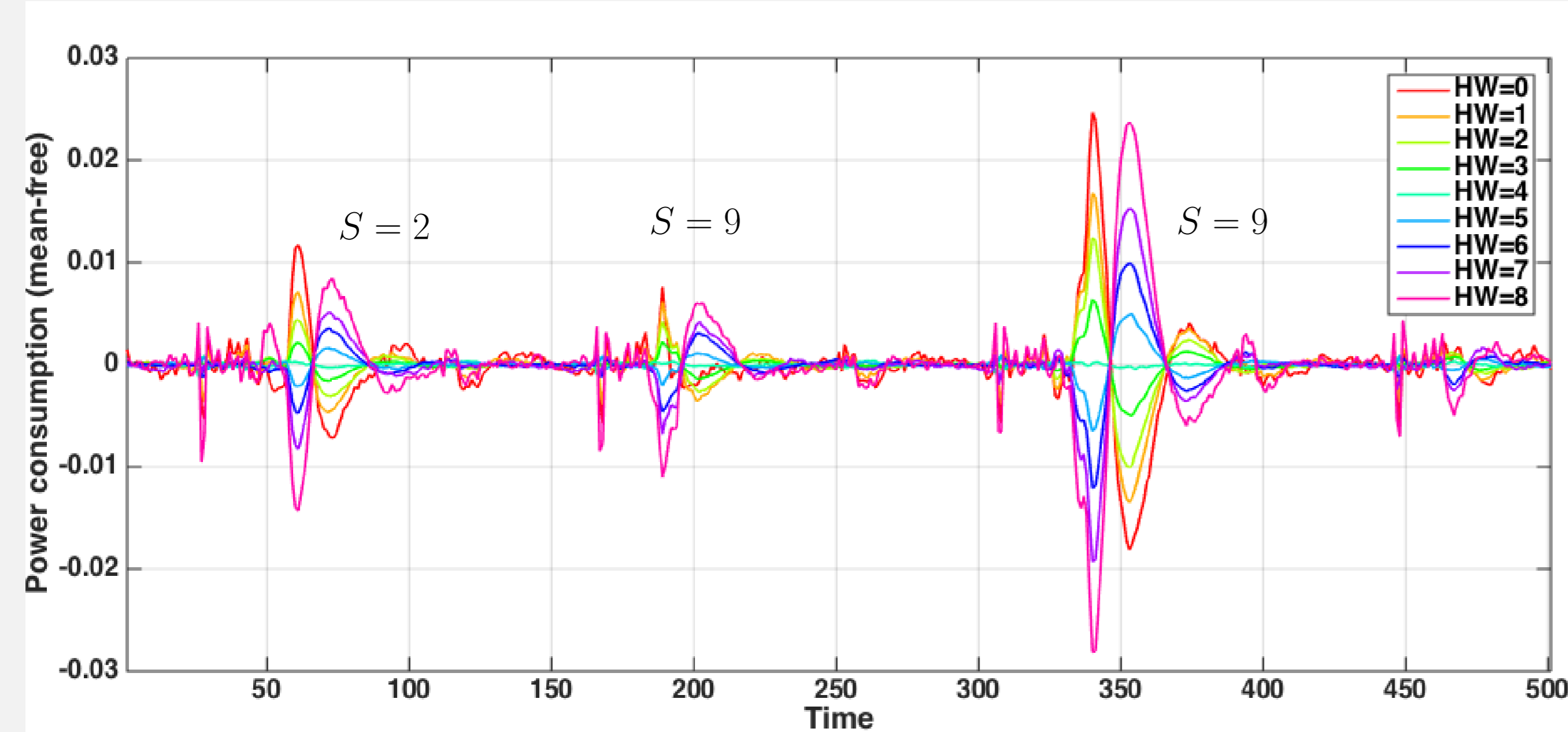
(b) Mean power consumption for each Hamming weight class
