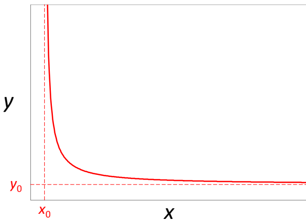
Figure 2. A decreasing and convex trade-off function with asymptotes at x_0 and y_0 .
