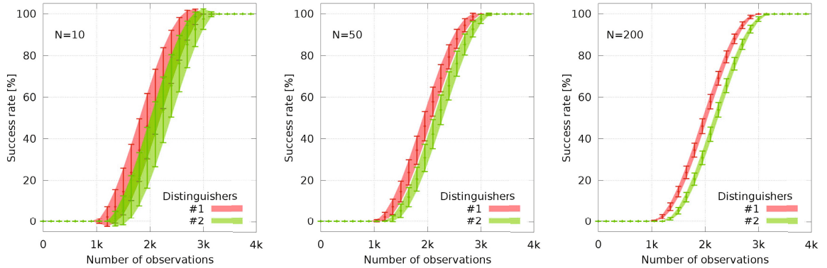
Fig. 1. Examples of success rates errors (Eqn. (3)) for various numbers of experiments
