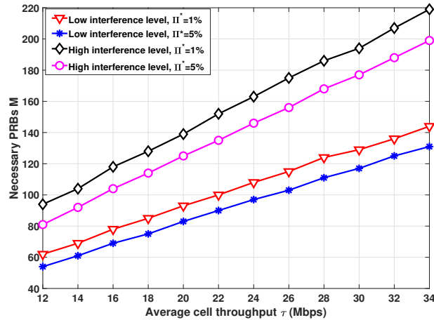
Figure 8: Interference impact on dimensioned PRBs M .
