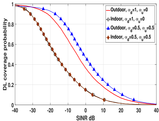
Figure 10. Small-cells DL coverage probability : 2b = 3.5 , k = 0.4 and \lambda = 10 small-cell/ \text{km}^2 .
