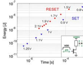
Fig. 4. Simulated SET/RESET energy versus switching time for various voltage ( V_{\text{DDH}} ) across the cell shown in the inset.
