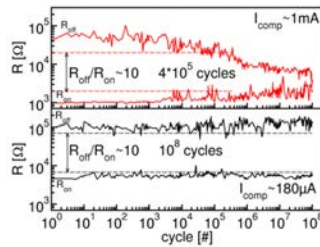
Fig. 2. Experimental pulse cycling endurance test for a SET compliance current ( I_{\text{COMP}} ) of 1mA (top) and 180μA (bottom).
