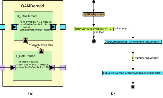
Figure 4: The SysML Composite (a) and Activity (b) diagrams for operation 64QAM Demodulation.
