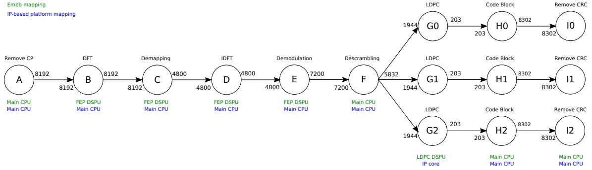
Figure 7: The single-rate SDF graph of the 5G decoder in Fig. 3 (tokens are expressed in bytes).
