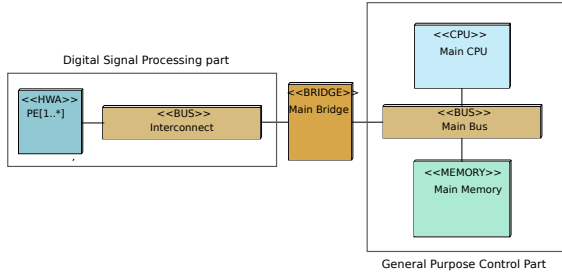
Figure 5: The UML Deployment Diagram of a generic instance of Embb and of the hardware IP-based platform.
