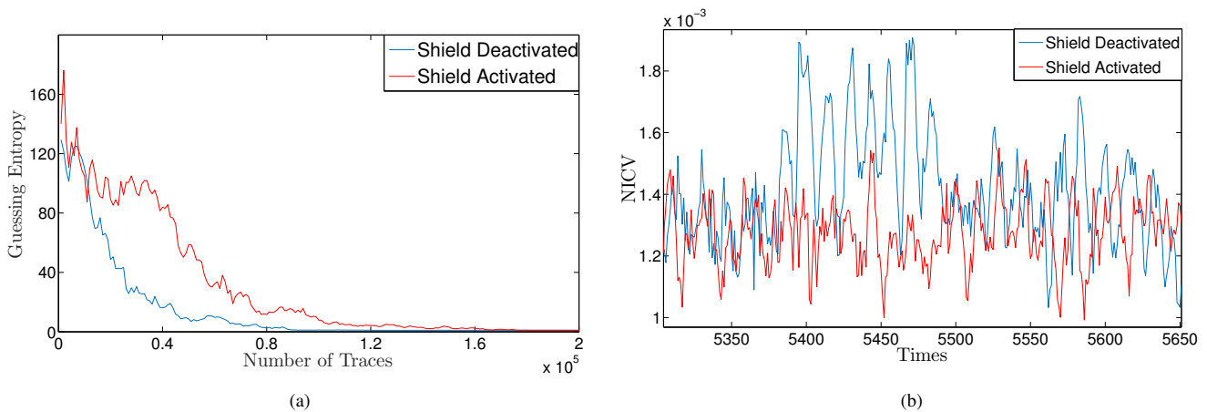
Fig. 13. (a) Guessing Entropy computation for AES with activated/deactivated shield. (b) NICV computation for AES with activated/deactivated shield.
