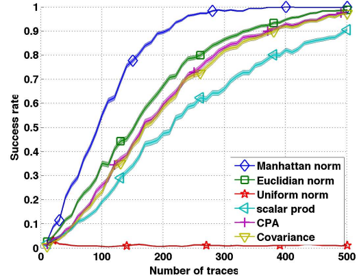
(f) Laplacian Noise, \sigma = 6
