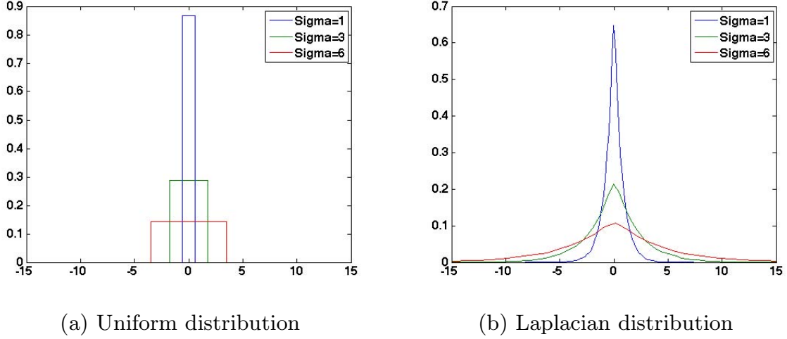
Fig. 2. Probability distributions for \sigma \in \{1, 3, 6\}
