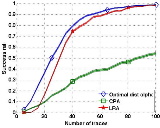
(c) \sigma_\alpha = 2, \sigma = 3
