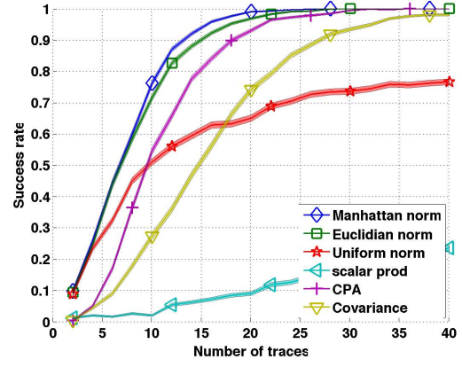
(b) Laplacian Noise, \sigma = 1
