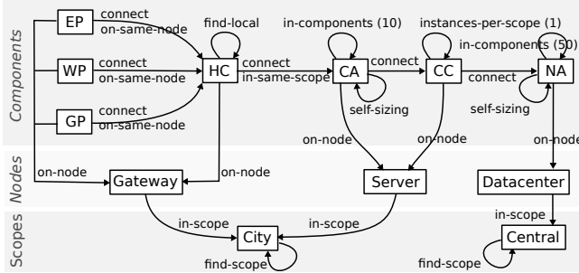
Figure 5. Complete constraints graph for use case archetype
