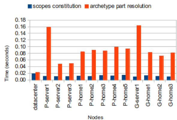
Figure 6. Average times of scope and archetype part resolution
