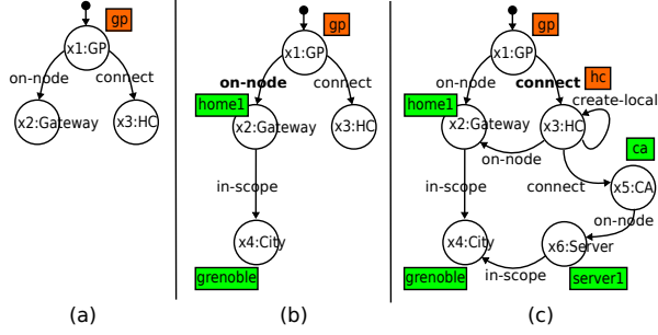
Figure 4. Example of Constraint Resolution Graph
