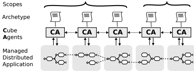
Figure 1. Cube agents managing distributed application
