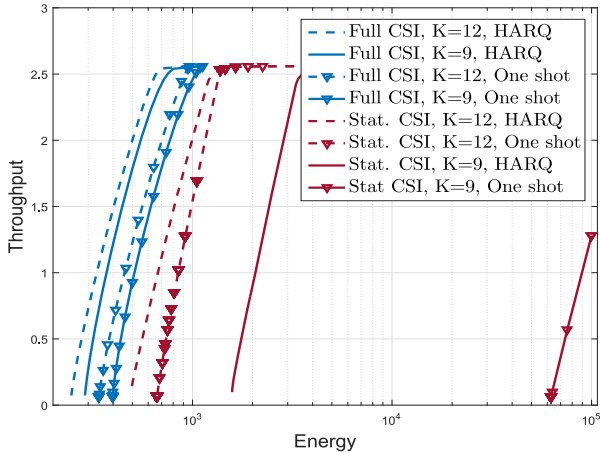
Fig. 4: Throughput versus energy for \alpha \in [0, 1] when HARQ or one shot transmission is used, with E_b = P_{\max} N_\ell , P_{\max} = 1000(30\text{dB}) , and N_\ell = 4000 .
