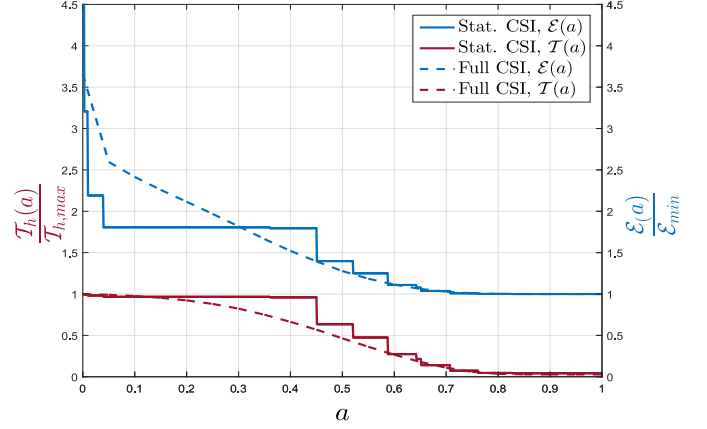
Fig. 2: Throughput and energy relative to their optimal value for Rician channel with K = 7 dB, B = 32 Bytes, \varepsilon_{\text{rel}} = 10^{-5} and maximum energy E_b = P_{\max} N_\ell with P_{\max} = 30 dB and N_\ell = 4000 .
