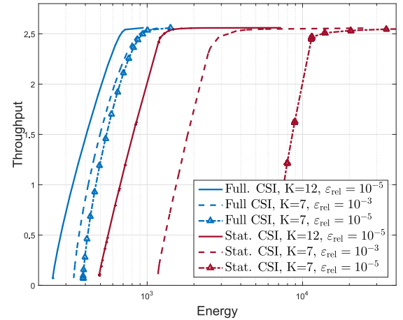
Fig. 3: Throughput versus energy for a \in [0, 1] , with E_b = P_{\max} N_\ell , P_{\max} = 30 dB, and N_\ell = 4000 .
