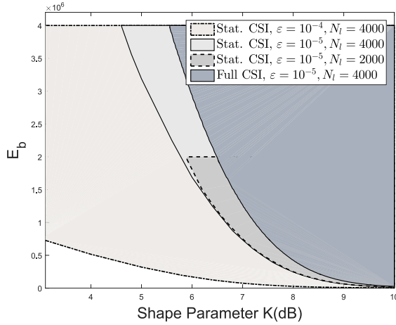
Fig. 1: Feasibility region for different channel, B = 32 Bytes, maximum energy budget E_b = P_{\max} N_\ell with P_{\max} = 30 dB.
