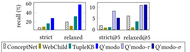
Figure 5: Recall evaluation.
