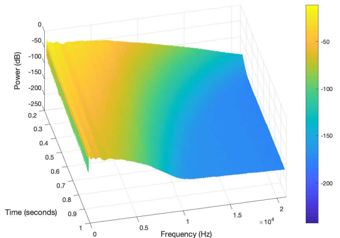
Fig. 20. Time-frequency power profile \mathcal{W}_{\gamma_i, i}(t, f) in the Great Hall
