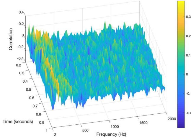
Fig. 22. Imaginary part of the time-frequency correlation \rho_{1,2}(t, f, \mathbf{x}_2 - \mathbf{x}_1) in the Great Hall
