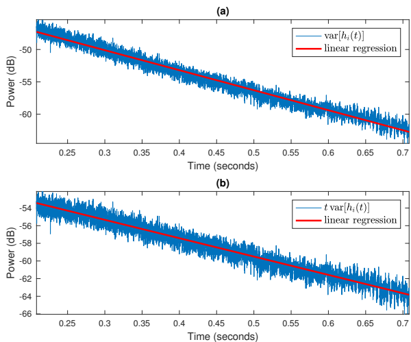
Fig. 8. Temporal power profile \text{var}[h_i(t)] in the classroom
