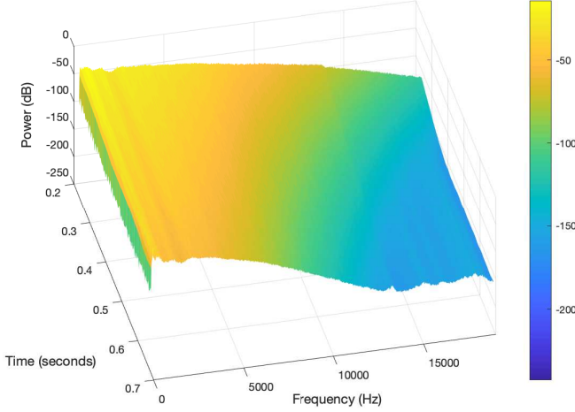
Fig. 9. Time-frequency power profile \mathcal{W}_{\gamma_{i,i}}(t, f) in the classroom
