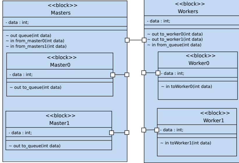
Figure 3: Task farm application: block diagram
