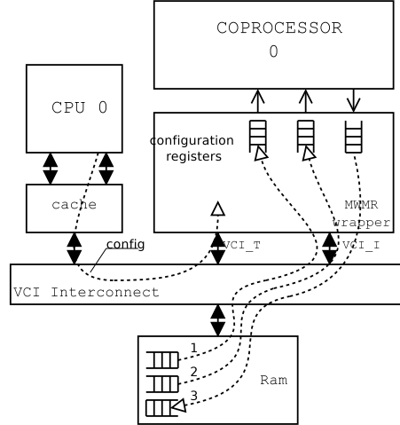
Figure 6: Co-processor interface
